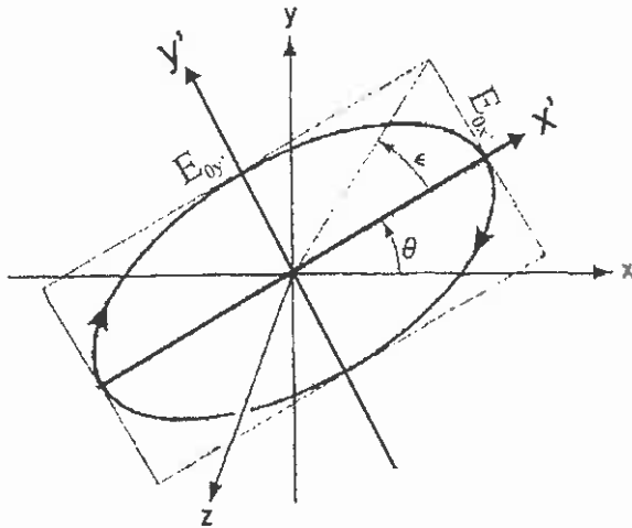
Figure Polarisation ellipse.
