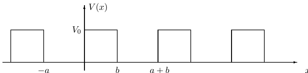
Figure 1: A one dimensional periodic box potential of period L = a + b .
