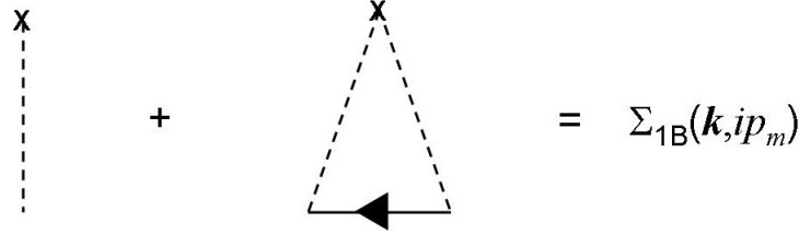
Figure 2: The approximation to the self-energy known as the first Born approximation.
