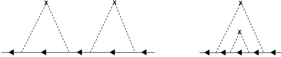
Figure 1: Two Feynman diagrams.
