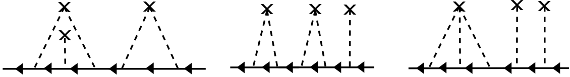
Figure 3: All inequivalent Feynman diagrams at order n = 5 with m = 3 impurity crosses that can be constructed from self energy diagrams up to order 3.
