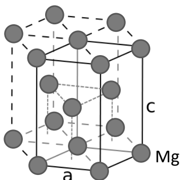
II - Mg
