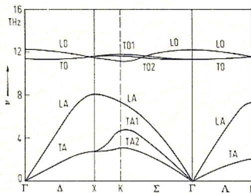
Phonon dispersion relation
