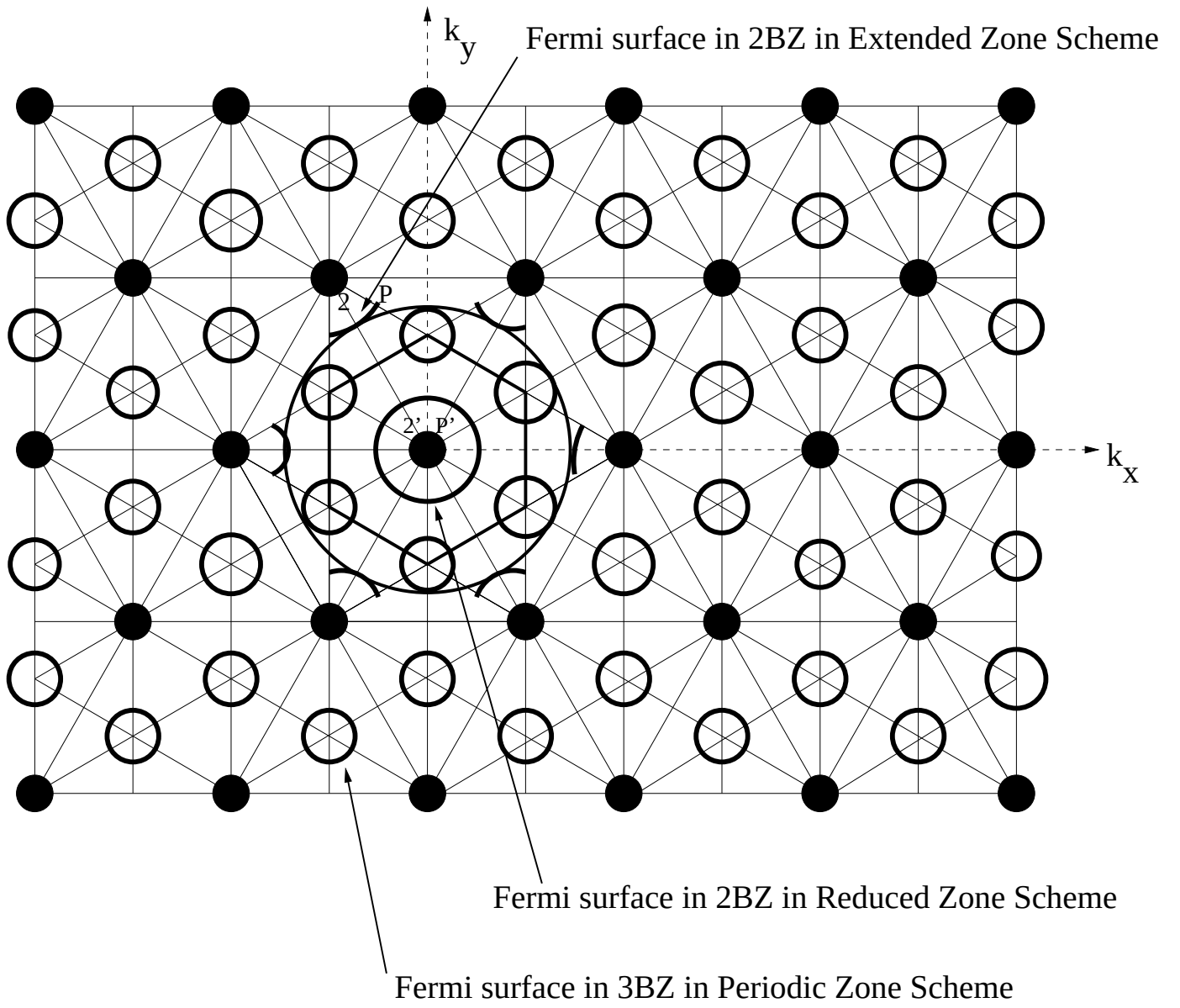
Figure 2: Fermi surface in hexagonal metal.
