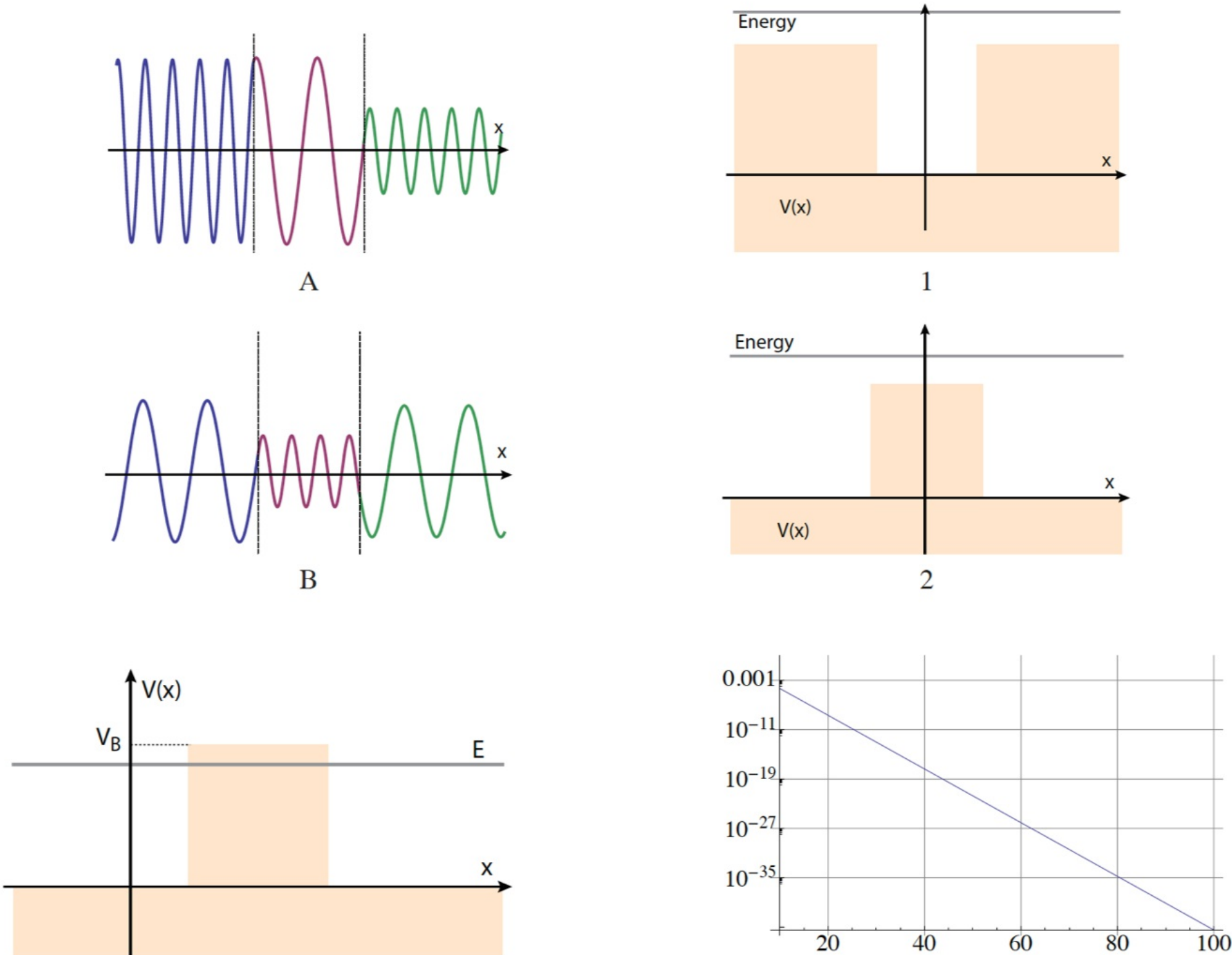
Figure 1: Left: Scattering potential. Right: e^{-x} .
