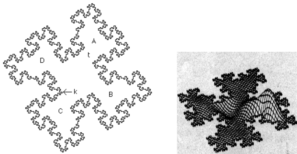
Figure 1: The boundary of the (quadratic Koch curve) fractal drum studied by Sapoval et al. [4]. Only the 3rd generation of the fractal is shown. The limiting curve for the shape has fractal (box-counting) dimension \ln(8)/\ln(4) = 3/2 .
