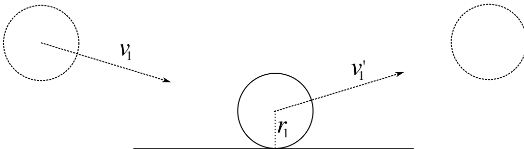
Figure 2: Collision between a particle and a wall.
