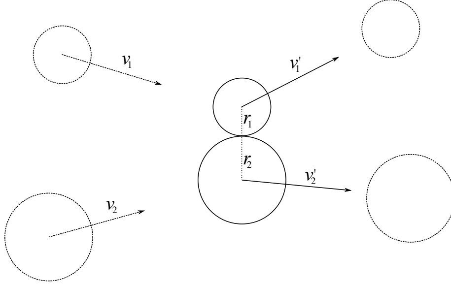
Figure 3: Collision between two particles.
