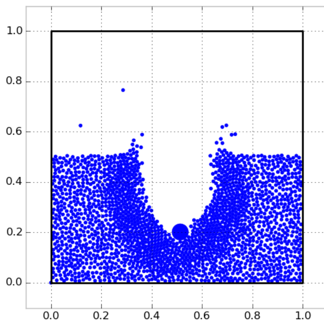
Figure 4: Example of crater formation.
