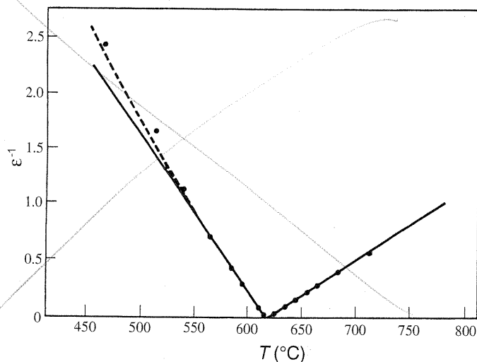
Fig. 3.4. LiTaO 3 in the region around the Curie temperature: Temperature dependence of the (inverse) dielectric constant (from Lines [20]).
