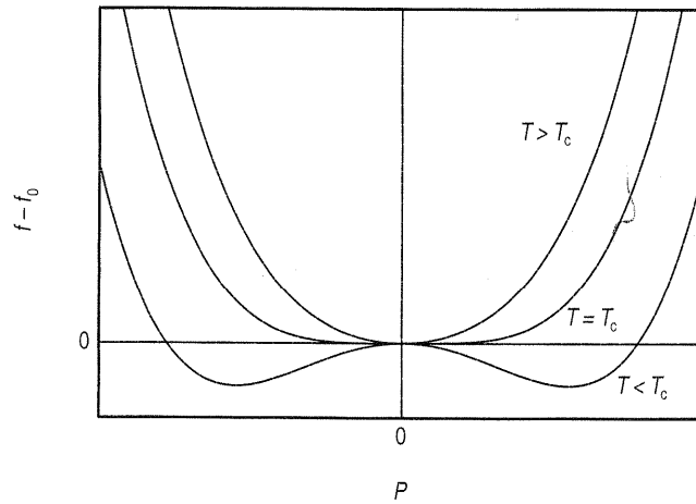
Fig. 3.5. The Landau expansion for the Helmholtz free energy density at the transition into the ferroelectric phase ( T = T_c ) as well as for temperatures above and
