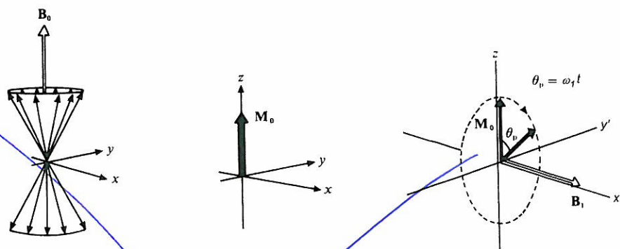
Fig. 2.26. System of spins in a static magnetic field \mathbf{B}_0 . Precession with the Larmor frequency ( left ) and resulting longitudinal magnetisation ( centre ). Rotation of the spin system by a transverse magnetic field \mathbf{B}_1 oscillating with the Larmor frequency. Precession in the rotating coordinate system x', y' ( right ).
