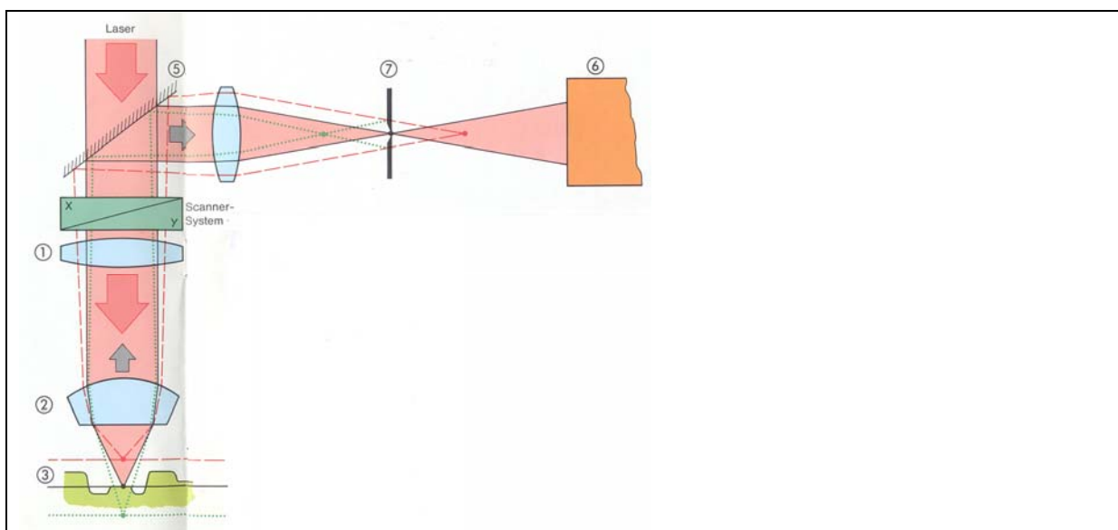
Figure 1: Setup for confocal laser scanning microscopy.
