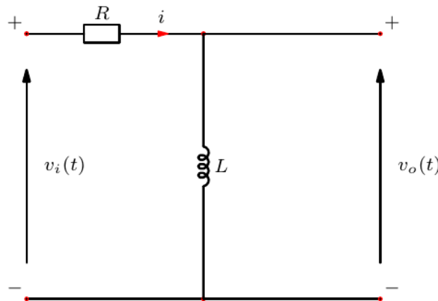
Figure 2: High pass filter circuit in Question 4
