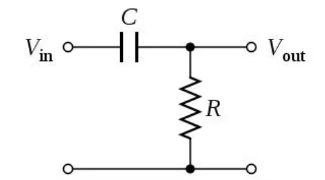
Figure 3: RC series circuit with output V_{\text{out}} = V_R(t) .
