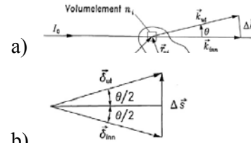
Figure 8. Schematic illustration of incident and scattered wave vectors ( \vec{k}_{in} and \vec{k}_{ut} ) and scattering vector \vec{\Delta k} (a) and the normalised wave vectors (b)
