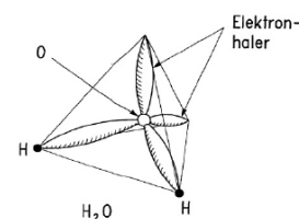
Figure 1. Schematic illustration of structure of water molecule
