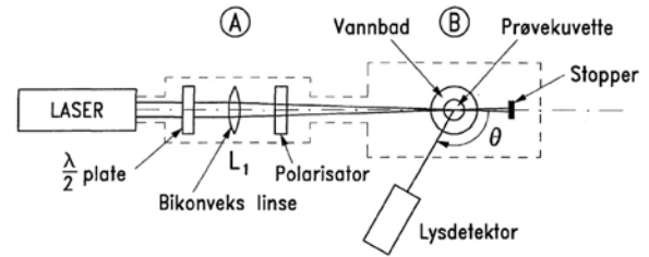
Figure 7. Schematic illustration of instrument for light scattering.
